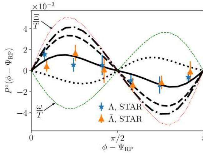
Local polarization
